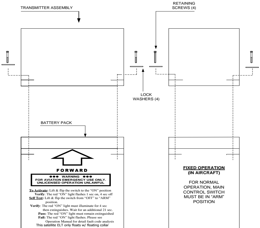
Figure 15: Battery Replacement for ELT Main Unit
