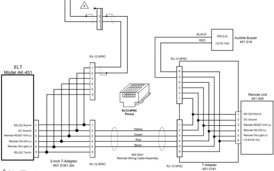
Figure 14.2a: Wiring Diagram for AK-451 with GPS Position and 3-inch T adapter with 4-wire interconnecting ELT Main Unit and Remote Switch Unit
