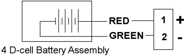
Figure 16: Battery Pack Replacement for ELT Main Unit (Actual View)
