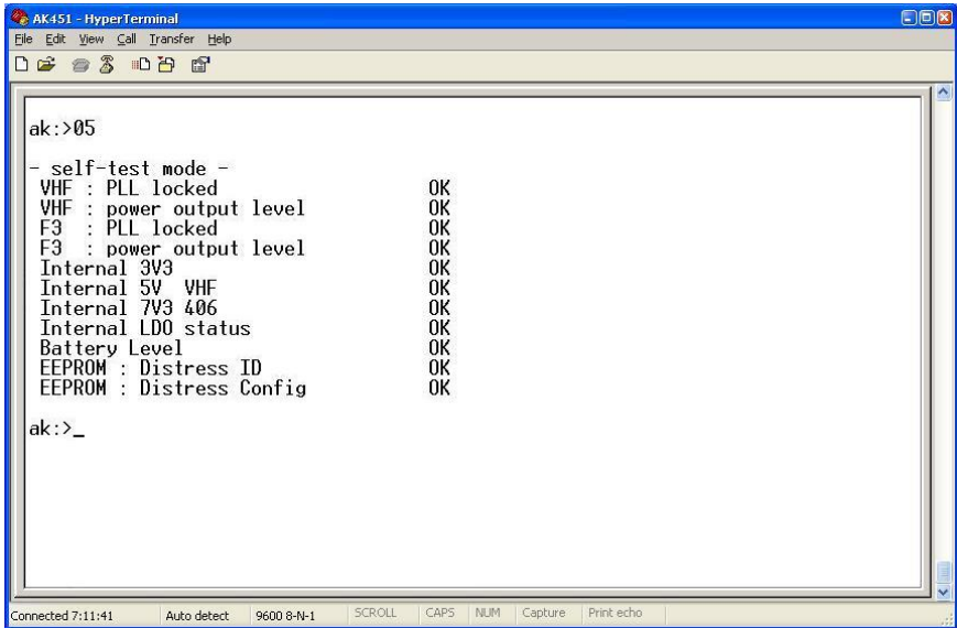
Figure 6: Maintenance Self-Test
