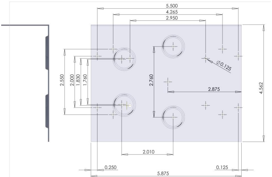
Figure 2.1.1: Optional Adapter Tray for ELT- (AF)(AP). P/N 450 013-1 for ACK Tech / Artex / Narco / Pointer ELT Retrofit
