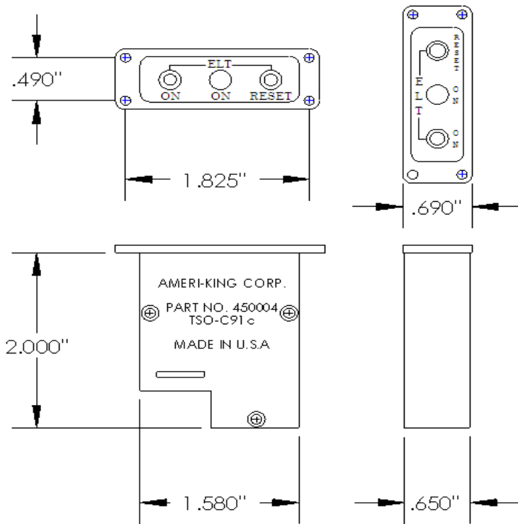
Figure 10: ELT Remote Switch Installation
