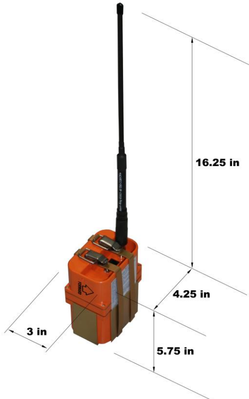
Figure 19: Automatic Portable-ELT (AP) with integral antenna Survival-ELT (S)
