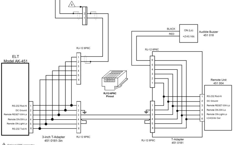
Figure 14.2b: Wiring Diagram for AK-451 with GPS Position and 3-inch T adapter with 2-wire interconnecting ELT Main Unit and Remote Switch Unit
