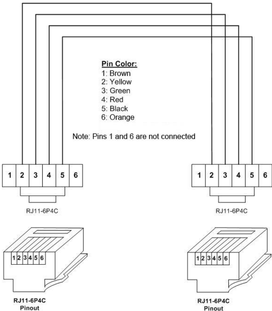
Figure 12.2: Interconnecting Wiring Cable between ELT Remote Unit and Main Unit, Part No. 4500041-4
