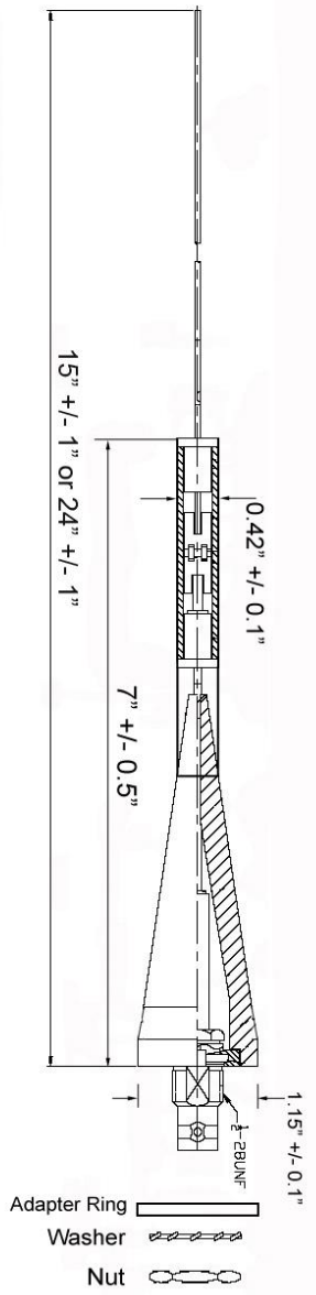
Figure 6: Whip Antenna (Model AK 451.017-1B)
